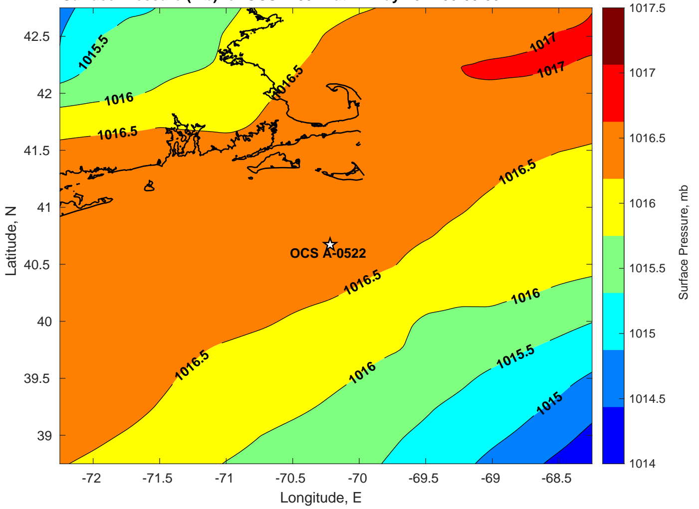
Surface Pressure (mb) for OCS A-0522 at 21-May-2024 00:00:00
